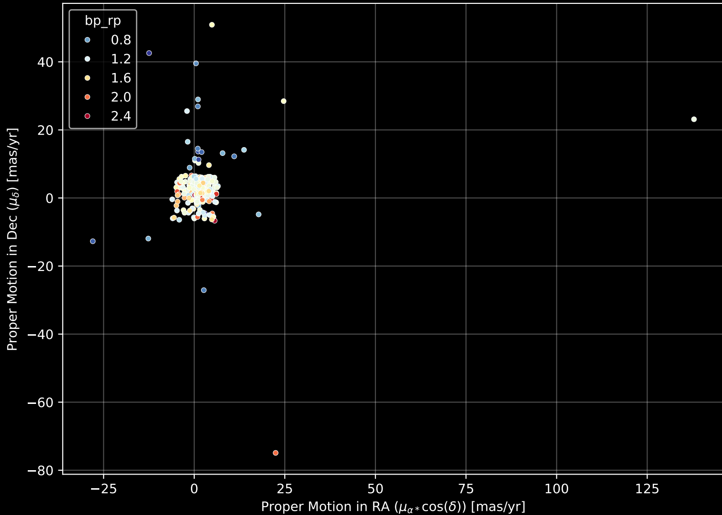
APOGEE DR17 Field: [299-28-C] Proper Motion Diagram (n= 217)
