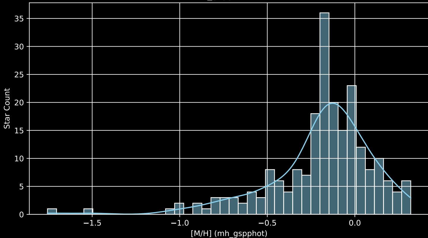
APOGEE DR17 Field: [299-28-C [M/H] (mh_gspphot) (n= 217)
