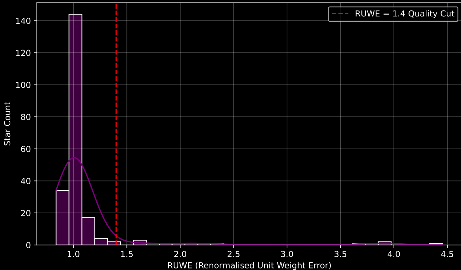
GAPOGEE DR17 Field [299-28-C] RUWE Distribution (n= 214)
