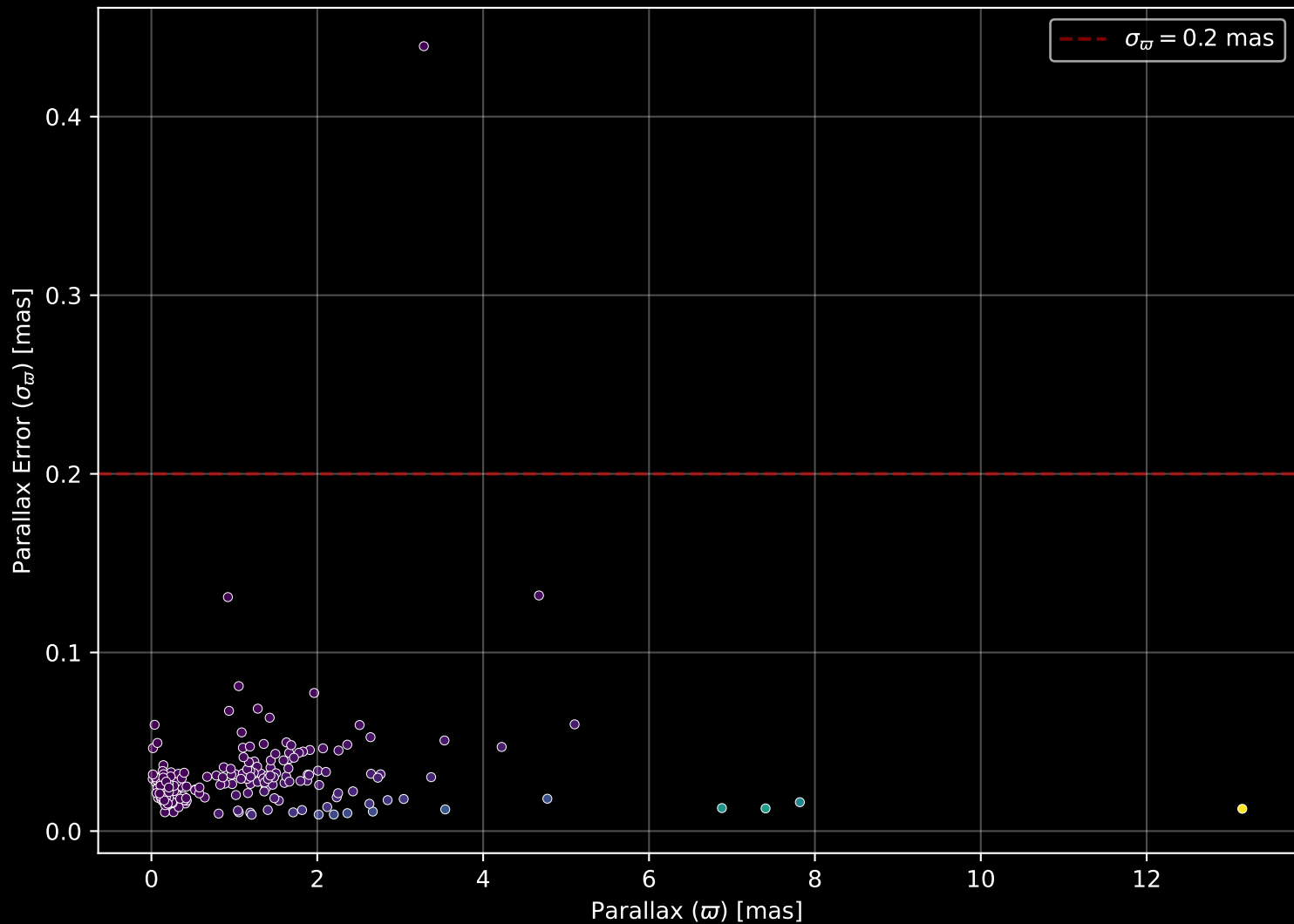
APOGEE DR17 Field: [299-28-C] Parallax Quality (n= 217)
