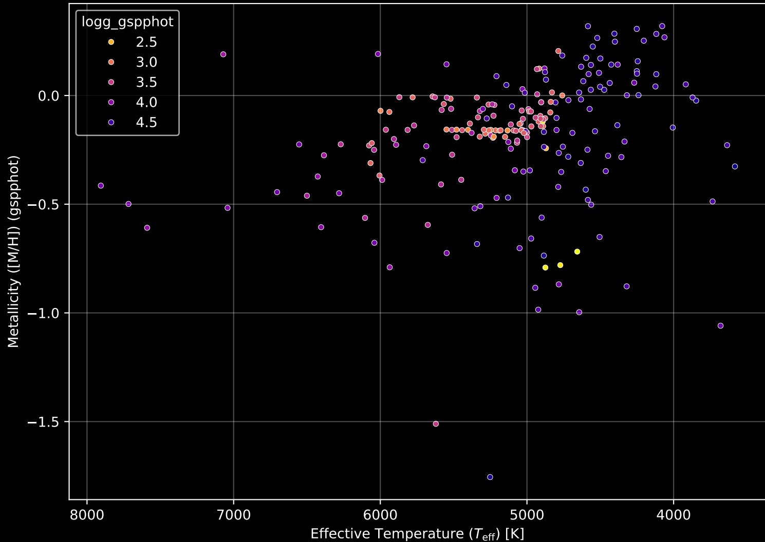
APOGEE DR17 Field: [299-28-C] Stellar Population Parameters (n= 217)
