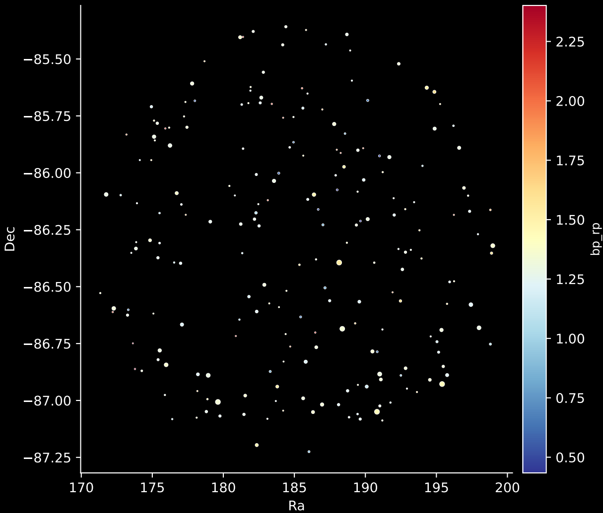
APOGEE DR17 Field: [299-28-C] Stars: 217
