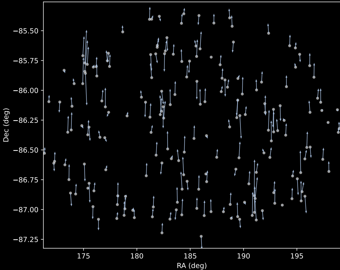
APOGEE DR17 Cluster 1 Proper Motion Vectors (n=191)
