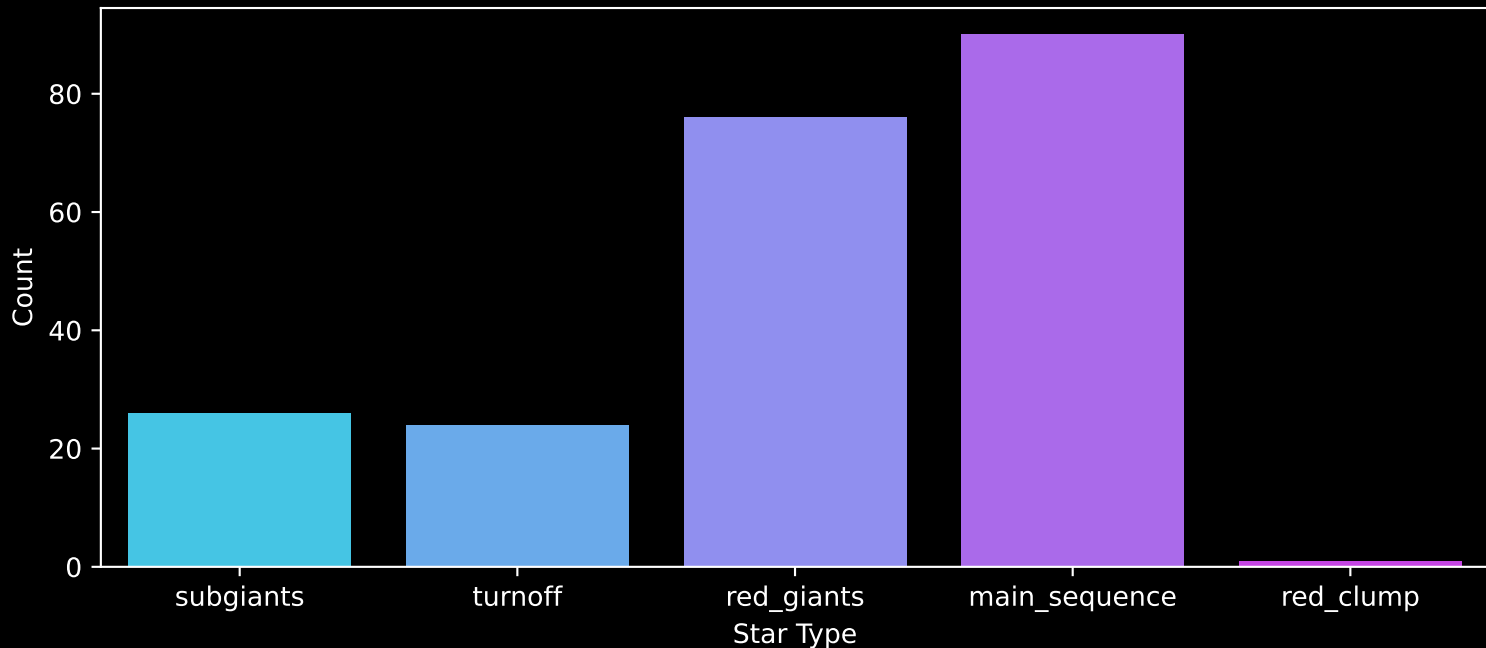
APOGEE DR17 Field: [299-28-C] Count plot of Star Type
